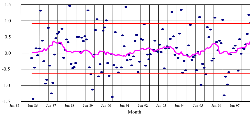
Figure 3.4A k = 1
