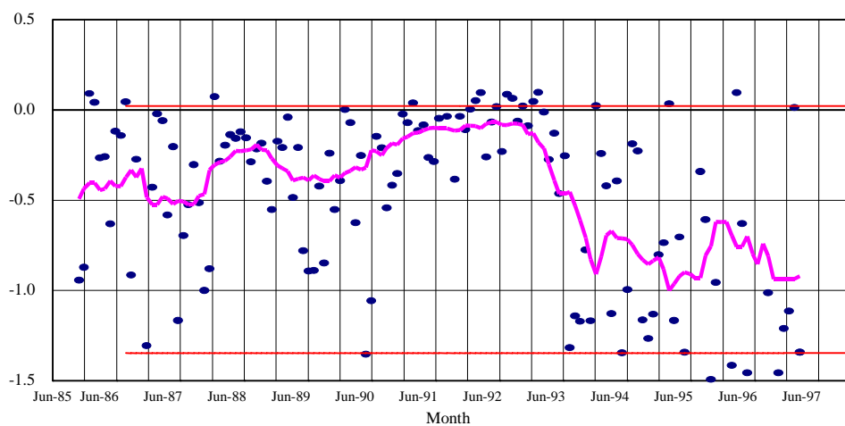
Figure 10.4C k = 10
