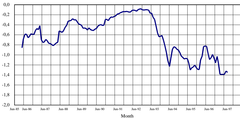
Figure 12.4C k = 10
