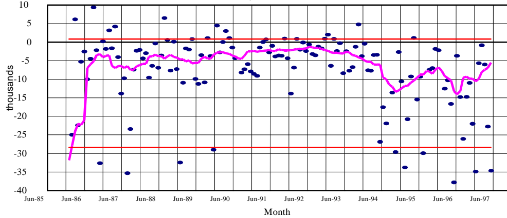
Figure 2.4C k = 10
