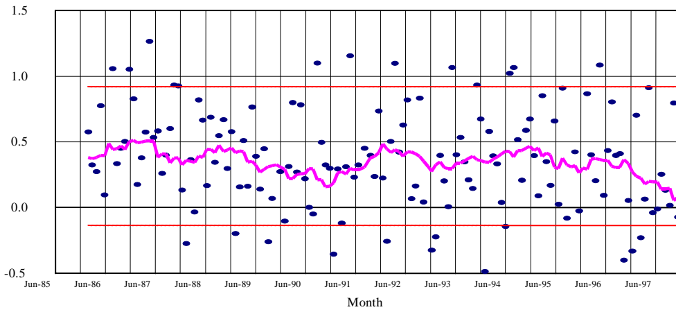
Figure 11.2B k = 4
