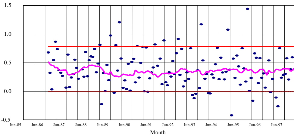
Figure 11.2C k = 10
