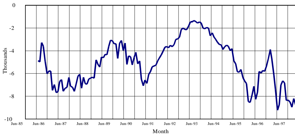
Figure 4.4A k = 1
