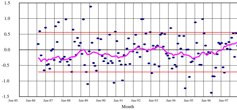
Figure 3.3C k = 10
